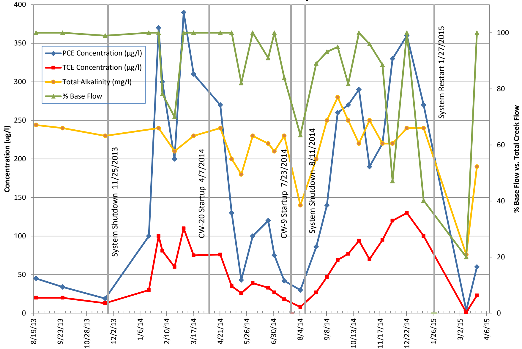
FIGURE 3.5-22 SW-17 Concentration vs Time compared to % Baseflow
